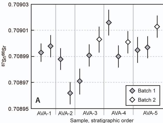
Appendix 8. A: Sr isotopic results plotted in stratigraphic order. B: Sr isotopic results ordered by ^{87}\text{Sr}/^{86}\text{Sr} value. Error bars on Sr ratios reflect 2\sigma analytical errors.
